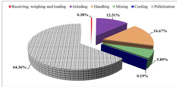
Fig. 4: The percentages of energy consumption in manufacturing large animal feed pellets.
