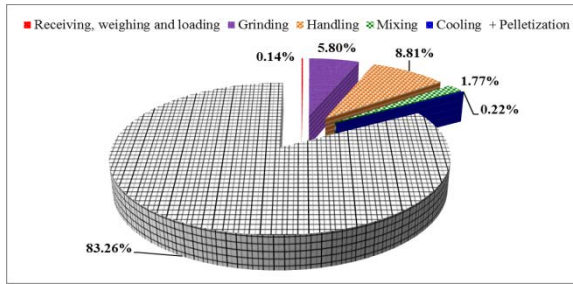
Fig. 3: The percentages of energy consumption in manufacturing poultry feed pellets.
