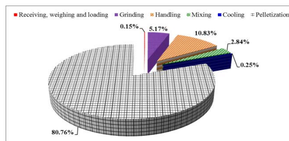
Fig. 2: The percentages of energy consumption in manufacturing rabbits feed pellets.
