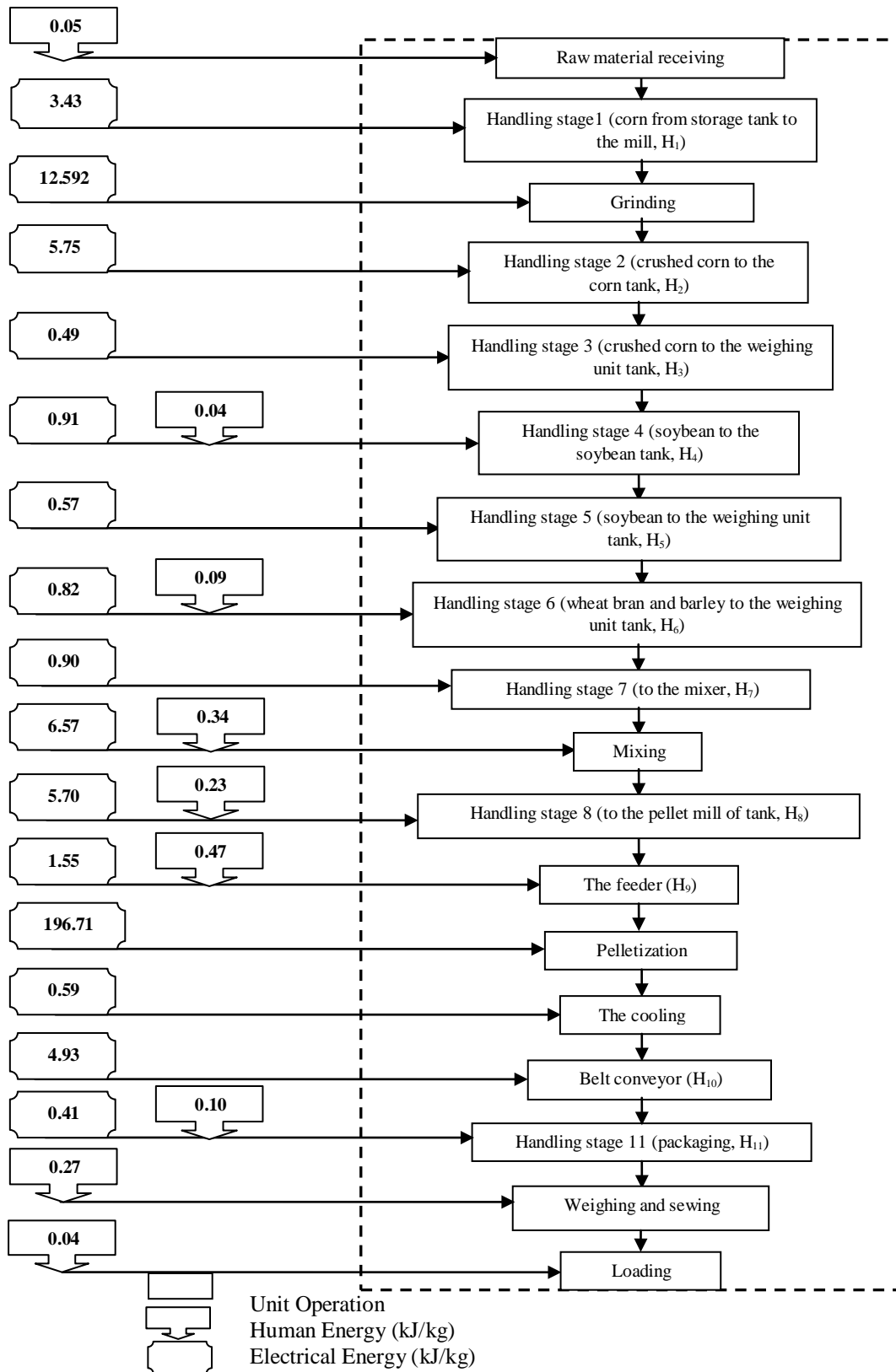
Fig. 5: Energy flow diagram of manufacturing processes of rabbits feed pellets.
