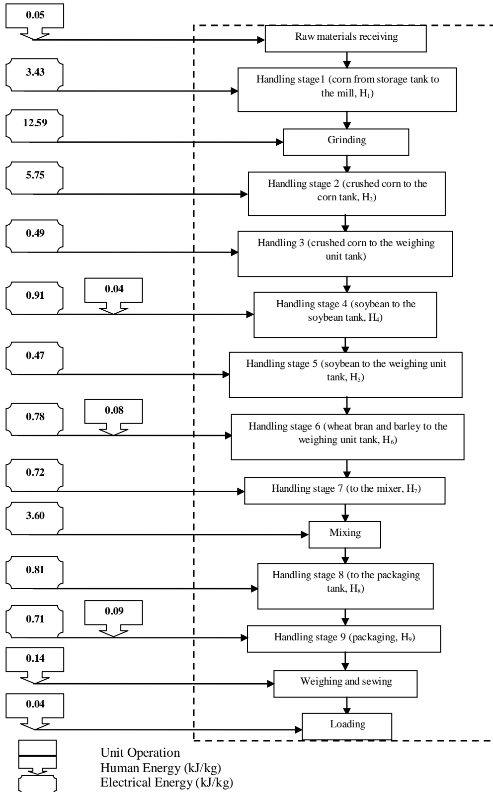
Fig.8: Energy flow diagram of manufacturing processes of large animal crushed feed.
